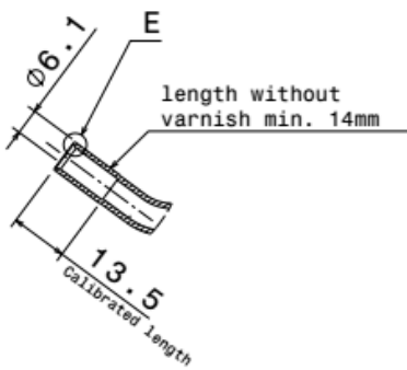
Section B-B Discharge tube
