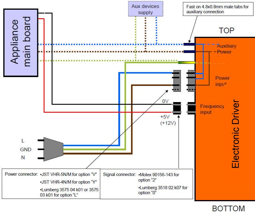
Frequency control connection example #1
